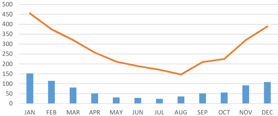
Comparison Balboa Heater to XC Heat Pump at SPA
